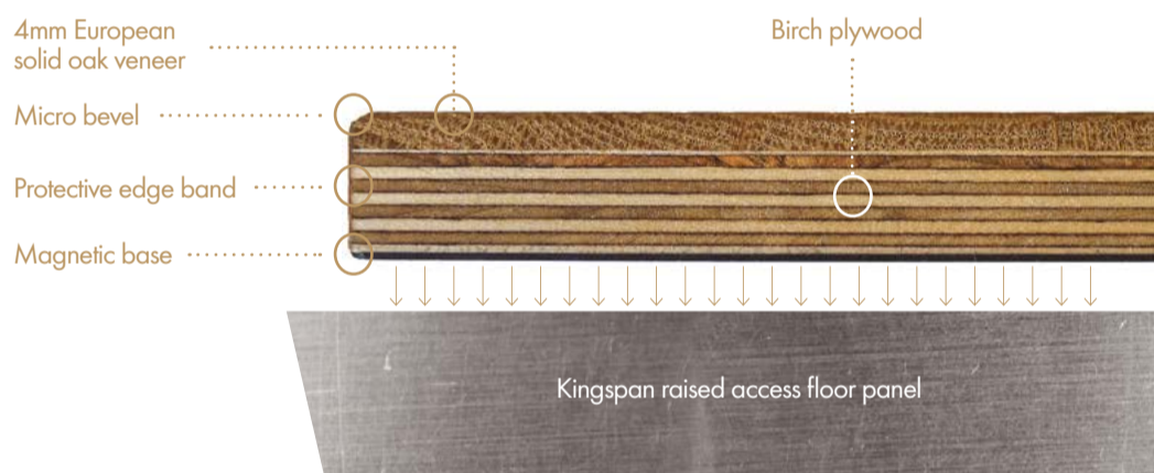
Kingspan raised access floor system
